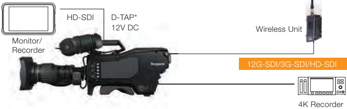
Example of System: Camera Head
